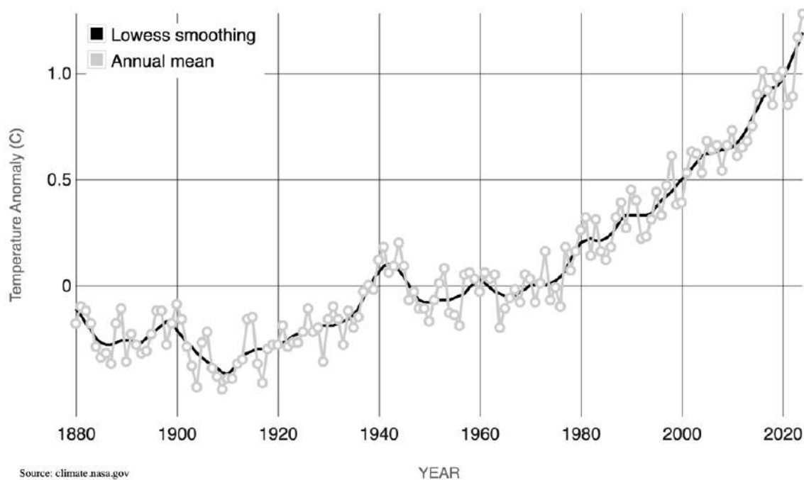
Figure 7. Average global surface temperature
